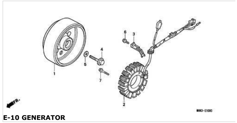
E-10 GENERATOR
