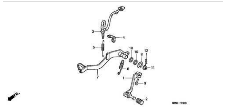
F-19 PEDAL
