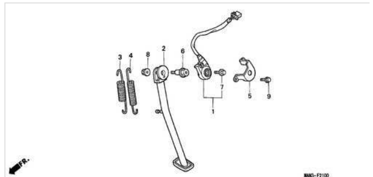
F-21 STAENDER
